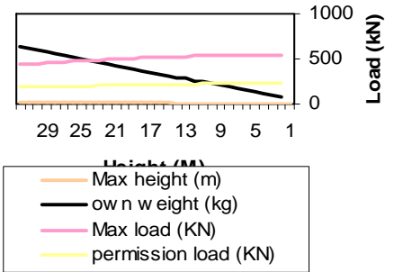
Shuttering tower
